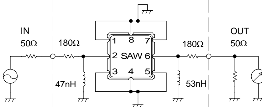
Fig.1 Measuring circuit
